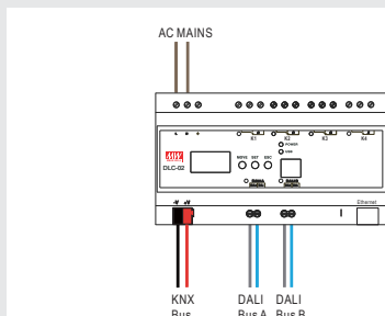
KNX gateway
